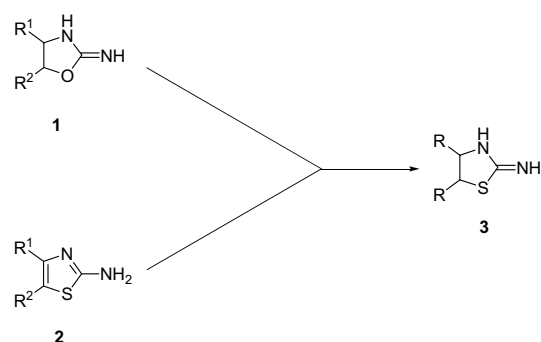
Chart 1. Molecular design of the 2-imino-1,3-thiazolidine derivatives 3 .
