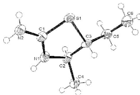
Figure 1. ORTEP view of X-ray structure of (4R,5R)\text{-14a} .
