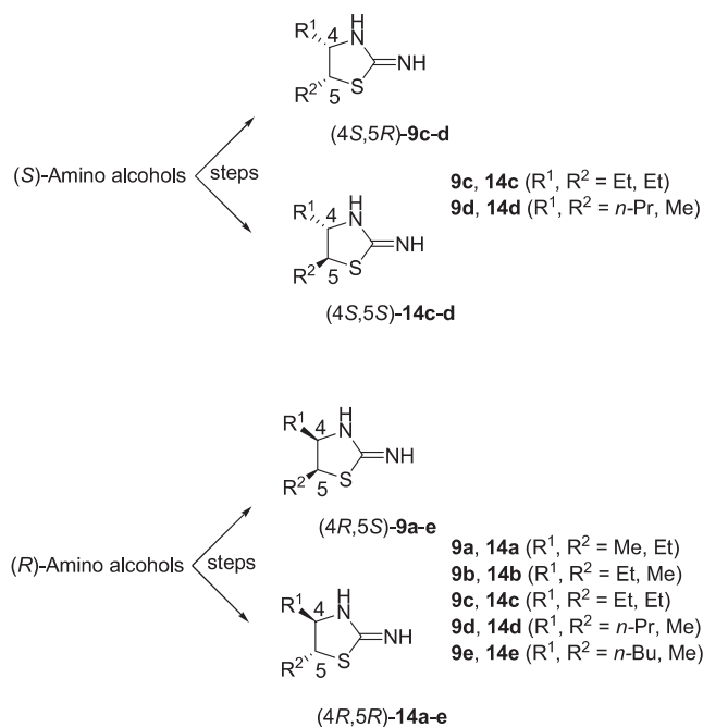
Scheme 2. Synthesis of the optically active 4,5-disubstituted 2-imino-1,3-thiazolidine derivatives as iNOS inhibitors. The reagents and conditions of synthesis for these derivatives are the same as those for the racemic derivatives.
