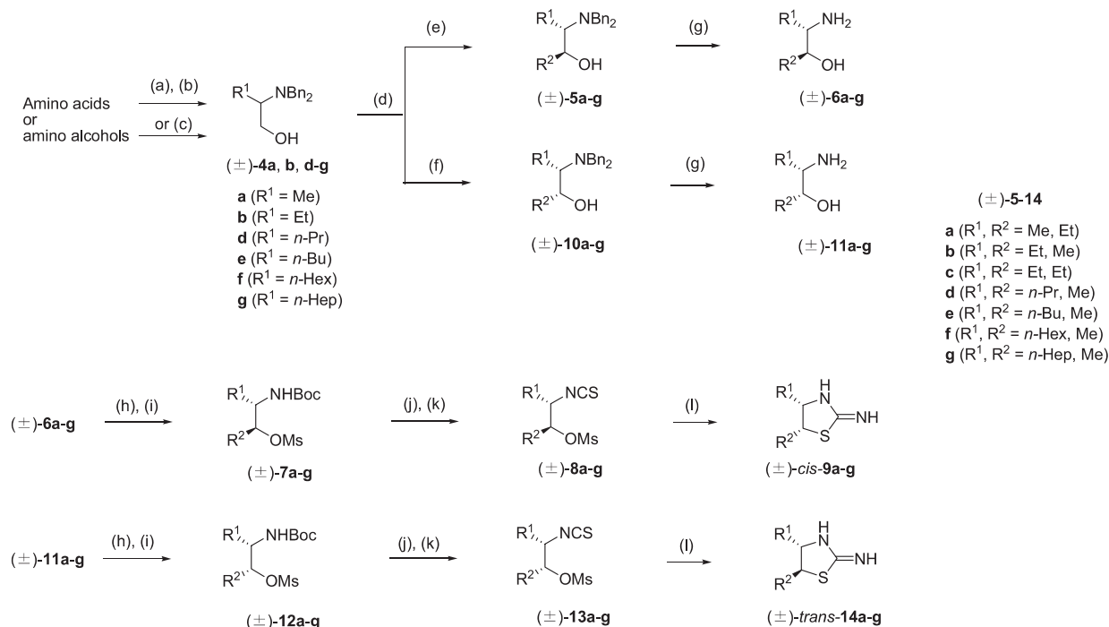
Scheme 1. Synthesis of racemic 4,5-disubstituted 2-imino-1,3-thiazolidine derivatives as iNOS inhibitors. Reagents and conditions: (a) BnBr, K 2 CO 3 , H 2 O, 100 °C; (b) LiAlH 4 , THF, rt; (c) BnBr, K 2 CO 3 , CH 3 CN, 60 °C; (d) Swern ox.; (e) (R 2 ) 2 Zn, toluene, 0 °C; (f) R 2 MgBr, THF, 0 °C; (g) H 2 , 20% Pd(OH) 2 -C, MeOH, rt; (h) Boc 2 O, CH 2 Cl 2 , rt; (i) MsCl, Et 3 N, CH 2 Cl 2 , 0 °C; (j) 30% HCl/EtOH, rt; (k) CSCI 2 , CaCO 3 , CHCl 3 , H 2 O, 0 °C; (l) 28% NH 3 aq, dioxane, 60 °C.
