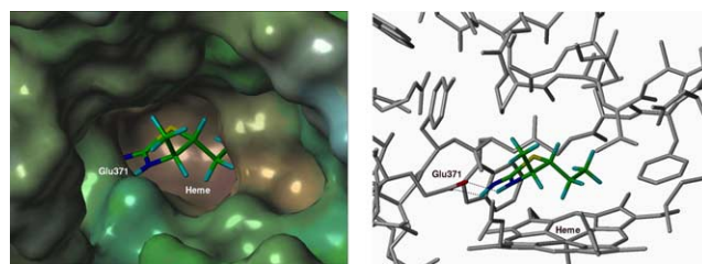
Figure 2. Left: Docking model of compound ( 4R,5R )- 14a in complex with iNOS in a surface representation. The compound resides in the small pocket above the heme. Right: Expected binding mode of ( 4R,5R )- 14a (green carbon atoms, yellow sulfur atom) in complex with iNOS oxygenase domain (gray). Interaction of ( 4R,5R )- 14a with iNOS is mainly due to a hydrogen bond between the amidine moiety of the inhibitor (light blue hydrogen atoms connected to blue nitrogen atoms) and the carboxylic acid group (red oxygen atoms, residue of Glu371). In addition, interaction of the sulfur atom of ( 4R,5R )- 14a with the iron atom of heme may be expected.
